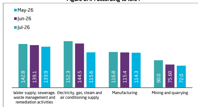
Figure3. Annual growth rate of sub-indices according to ISIC4-JULY 2026
